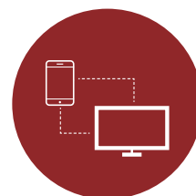
Communication Tools
